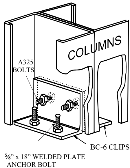
ATTACHMENT DETAIL
