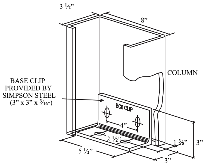
DIMENSION DETAIL
