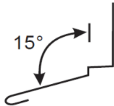
PARAPET HIGH 3:12 EAVE TRIM [D]
