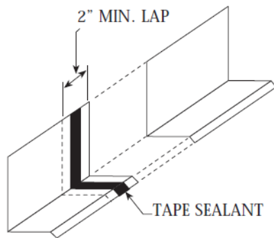
BASE TRIM DETAIL
